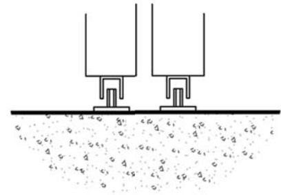
SECTIONAL VIEW BOTTOM FIXER
