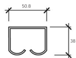
SECTIONAL TOP TRACK VIEW Aluminum Profile
