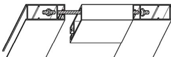
SECTIONAL FRAME VIEW SUS304 Stainless Steel Screw
