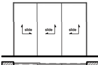
2 track 3 leaves
