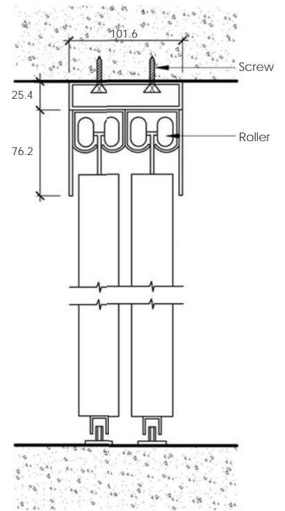
SIDE SECTIONAL VIEW
