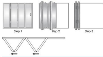
4 Door Series No. of Panel 4 + 0
