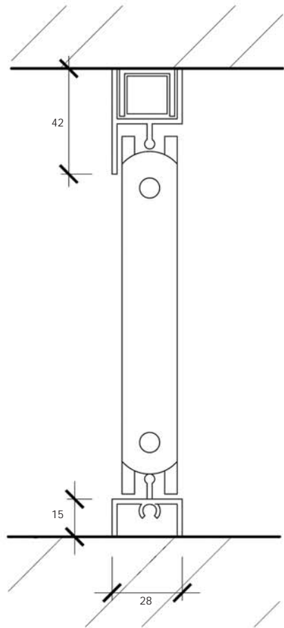
SIDE SECTIONAL
