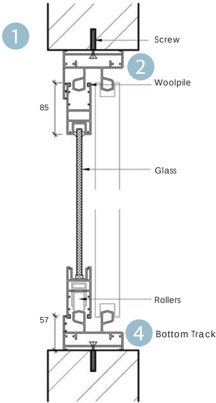
SIDE SECTIONAL
