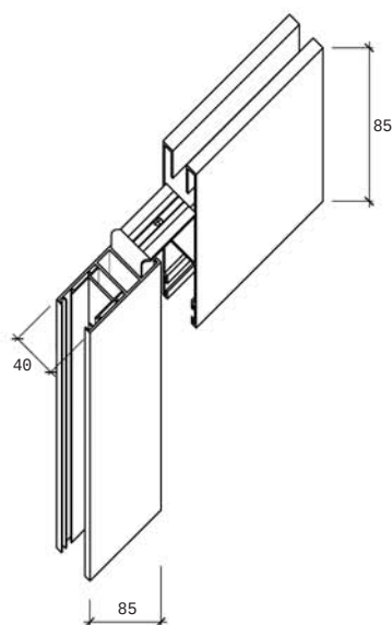
SIDE SECTIONAL
