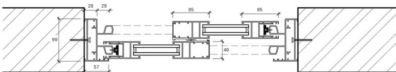
TOP SECTIONAL VIEW
