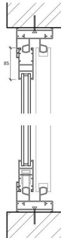
SIDE SECTIONAL
