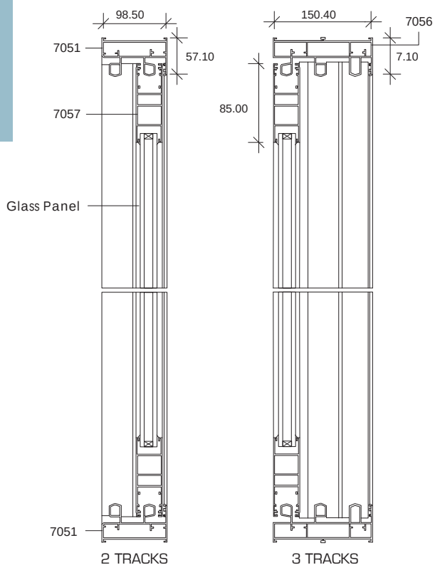
SIDE SECTIONAL
