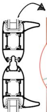
Handle Option1 Straight Sleek Hidden Handle
