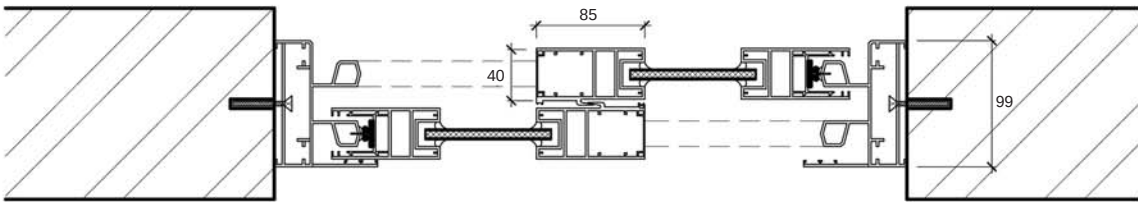
TOP SECTIONAL VIEW
