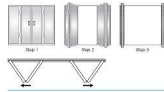
4 Door Series No. of Panel 2 + 2
