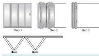
4 Door Series No. of Panel 4 + 0
