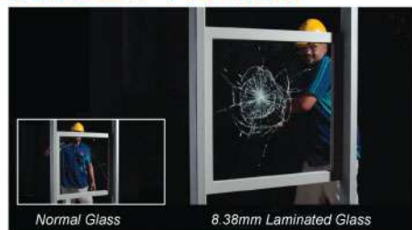
Normal Glass 8.38mm Laminated Glass IMPACT STRESS TEST (Baseball Bat and Steel Hammer)
