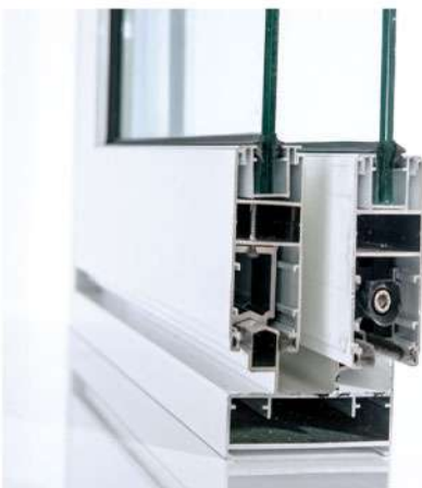
Aluminum Extrusion
