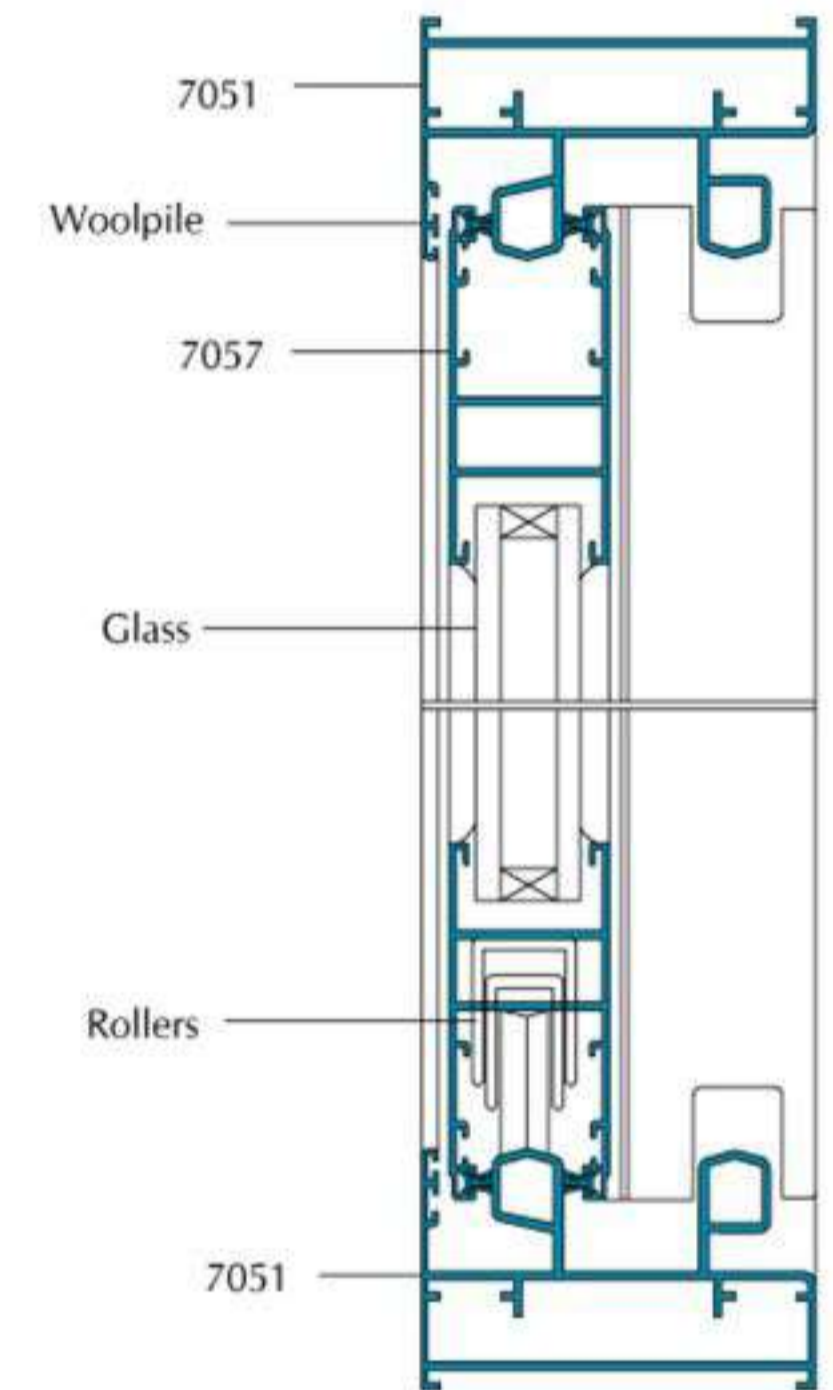
Vertical Section
