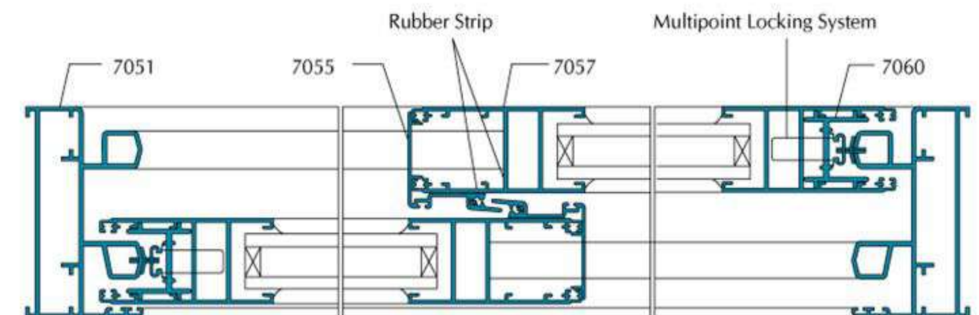
Horizontal Section
