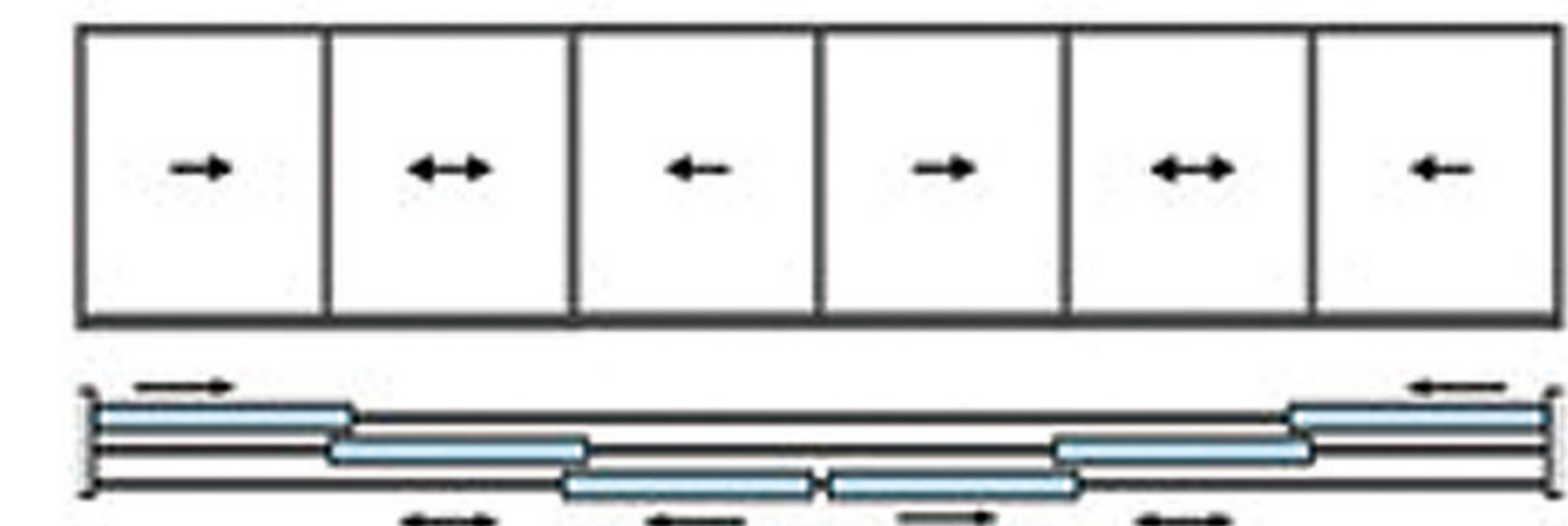
6-leaf 3 tracks
