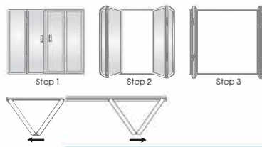
4 Door Series No. of Panel 2 + 2
