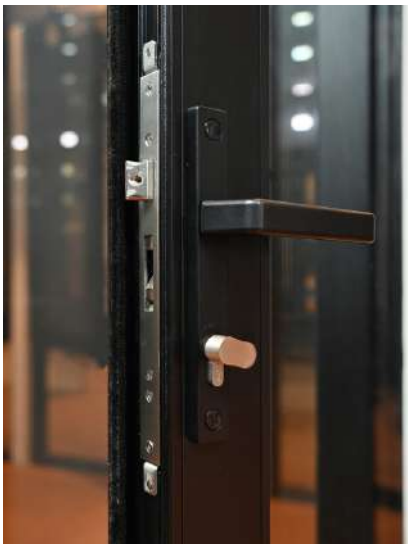
Multi-Point Lock
